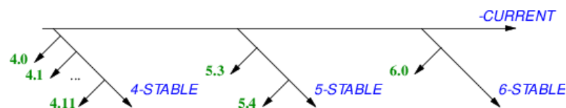
Figure 2. Les branches FreeBSD
